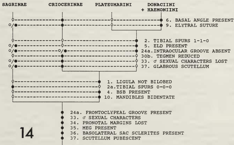
FIGURES 13, 14. Cladograms illustrating hypotheses of phylogenetic relationship of Donaciinae to Cricocerinae and Sagrinae. Apomorphic states indicated on diagrams. ● = apomorphic character states; ○ = plesiomorphic character states. 13, Hypothesis 1. The genus Atalasis is assumed to be the sister taxon to Donaciinae if apomorphic states in characters 1, 4, 6 and 10 in Cricocerinae are considered independently derived. 14, Hypothesis 2. The Cricocerinae is assumed to be the sister taxon to Donaciinae because characters 1, 4 and 10 could be considered synapomorphic for the grouping Cricocerinae + Donaciinae. This hypothesis requires reversal of character 6 in Plateumarini and most Sagrinae, or homoplasy of 6 between Donaciini and Cricocerinae. Reduction of character 2 is more easily derived from the cricocerine type than from the sagrine type.
